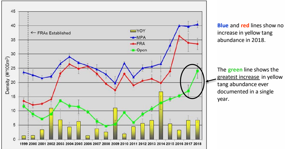
Figure 5. Overall changes in Yellow Tang density (Mean \pm SE) in FRAs, MPAs, and Open Areas, 1999-2018. Yellow vertical bars indicate mean density (MAY-NOV) of Yellow Tang YOY. YOY are not included in trend line data (DAR 2019a).
