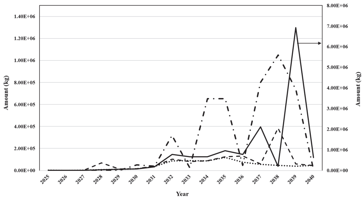
Figure 34. Aggregate disposal rates of steel from PV mounting structures across all scale for each island through 2040. Legend: O’ahu (solid line), Maui County (dashed line), Hawai’i County (dotted line), and Kaua’i (dashed-dotted line). For O’ahu, use right hand axis; for all other islands, use left hand axis.
