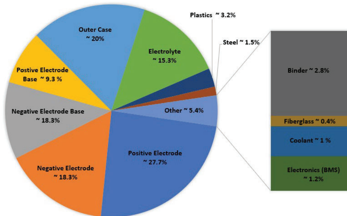
Figure 10. Averaged weight percentage of components in lithium-ion battery cells.
